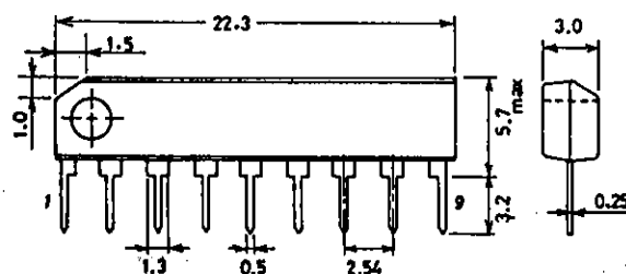
Package Dimensions 3017B unit: mm
